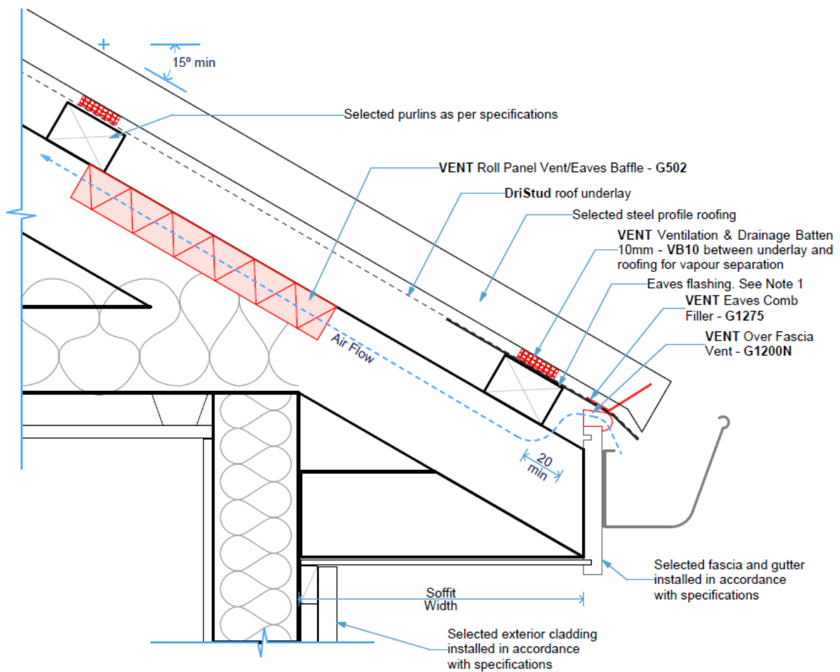
Figure A: G1275 Eaves Comb Filler. Installed with Over Fascia Vents
